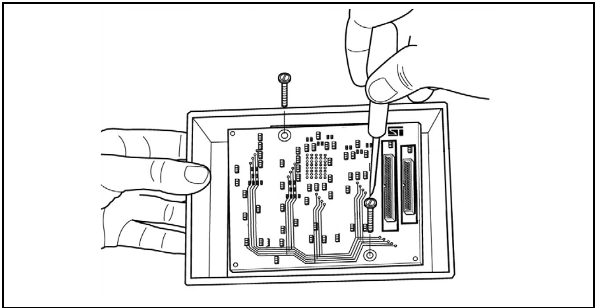
Figure 10: Removing the TEB screws
