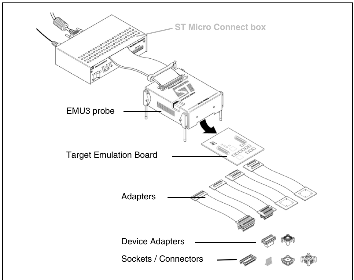
Figure 1: ST7MDTxxx-EMU3 terminology
